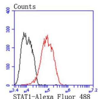
Fig. 4. Flow cytometric analysis of MCF-7 cells with STAT1 alpha antibody at 1/50 dilution (red) compared with an unlabelled control (cells without incubation with primary antibody; black). Alexa Fluor 488-conjugated goat anti rabbit IgG was used as the secondary antibody.
