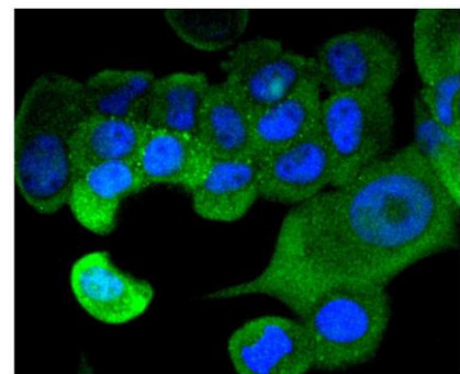
Fig. 2. ICC staining STAT1 alpha in MCF-7 cells (green). The nuclear counter stain is DAPI (blue). Cells were fixed in paraformaldehyde, permeabilised with 0.25% Triton X-100/PBS.
