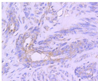
Fig. 3. Immunohistochemical analysis of paraffin-embedded human cervixuteri tissue using anti-STAT1 alpha antibody. Counter stained with hematoxylin.
