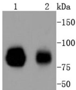
Fig. 1. Western blot analysis of STAT1 on different lysates using anti-STAT1 alpha antibody at 1/1,000 dilution. Positive control: Lane 1: HeLa; Lane 2: 293
